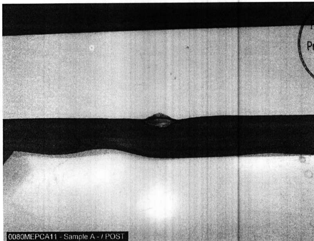
Figura 10. Sample A after the test
