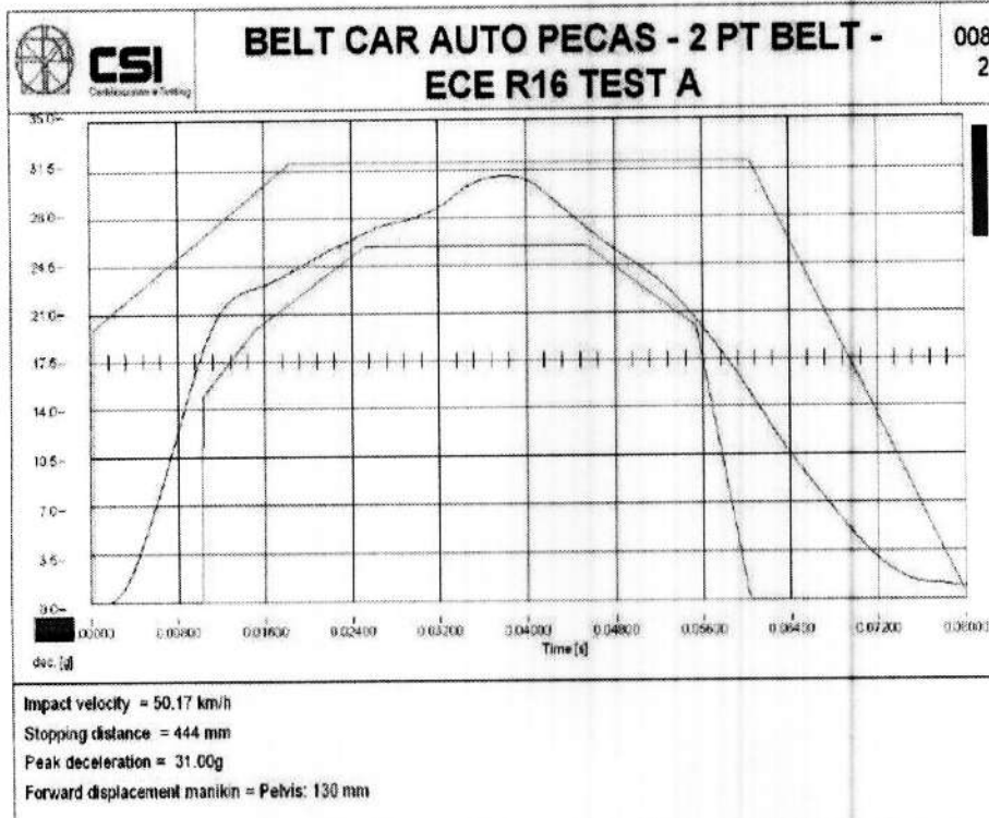
Figura 2. Sled deceleration profile during test A
